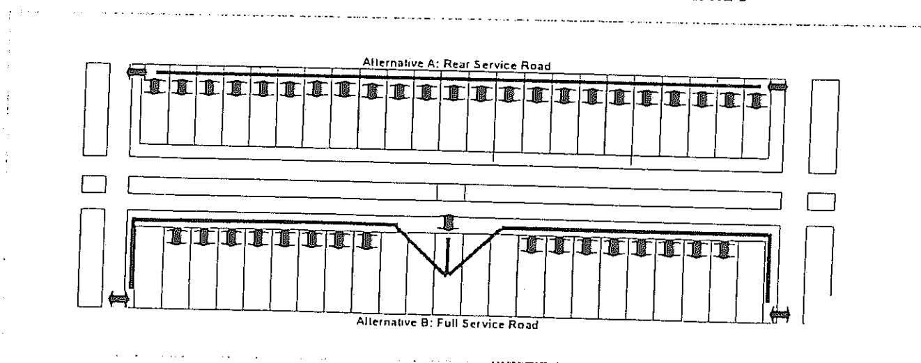
Figure 7.14: Service Road Alternatives A & B
