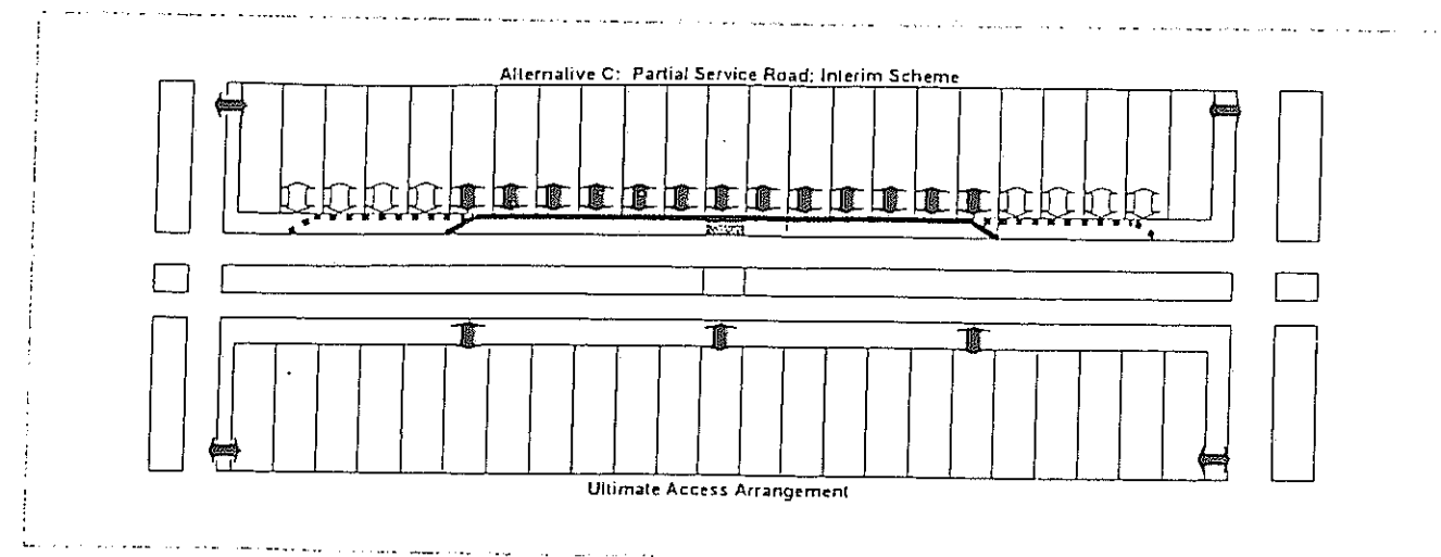
Figure 7.16: Interim Scheme for Alternative C
