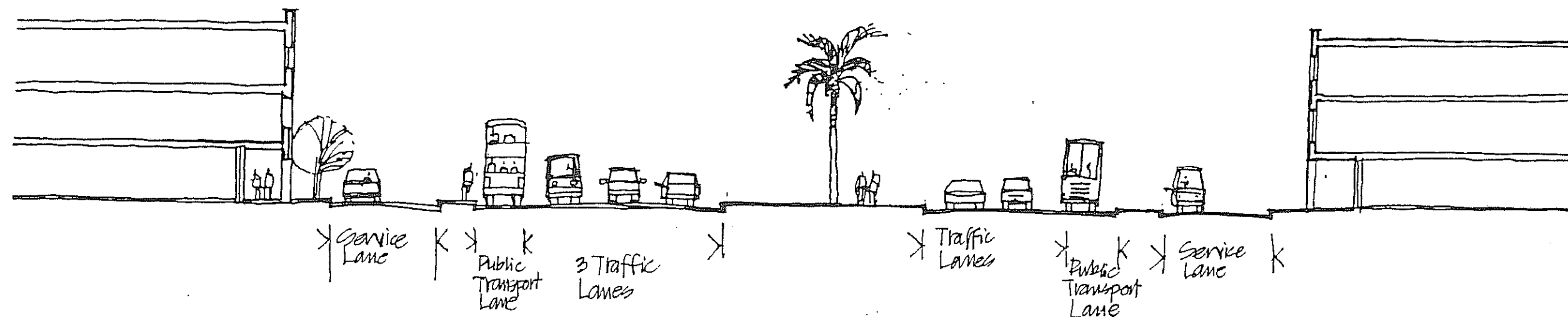
Alternative II B: 8 Lane Section with Service Lanes (3 traffic / mobility; 1 public transport)
