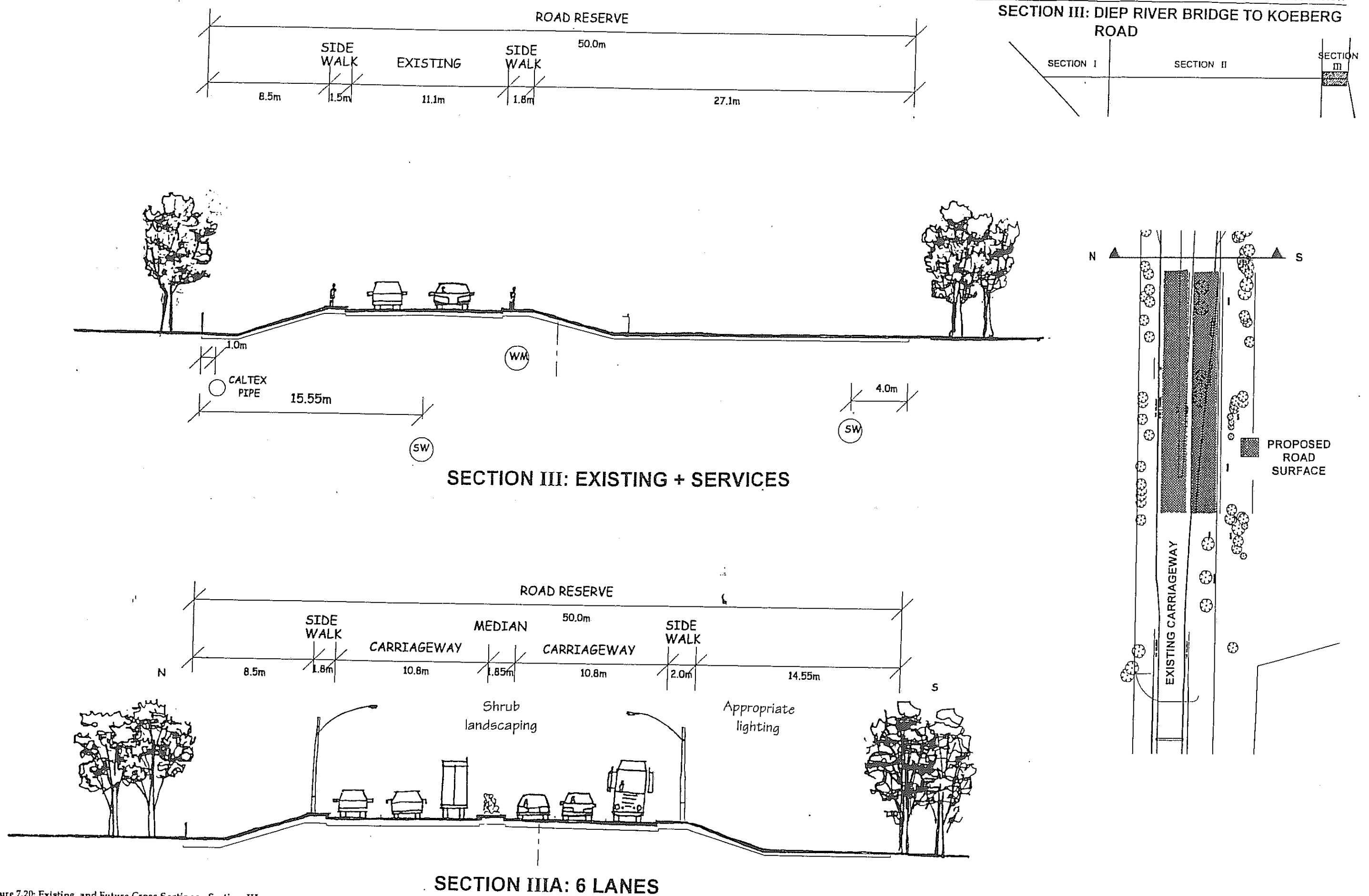
Figure 7.20: Existing and Future Cross Sections - Section III
